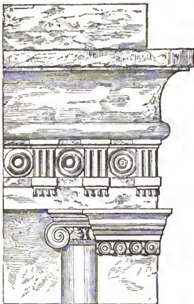
No. 5. — Angle of Tomb of Absalom. From De Saulcy.
